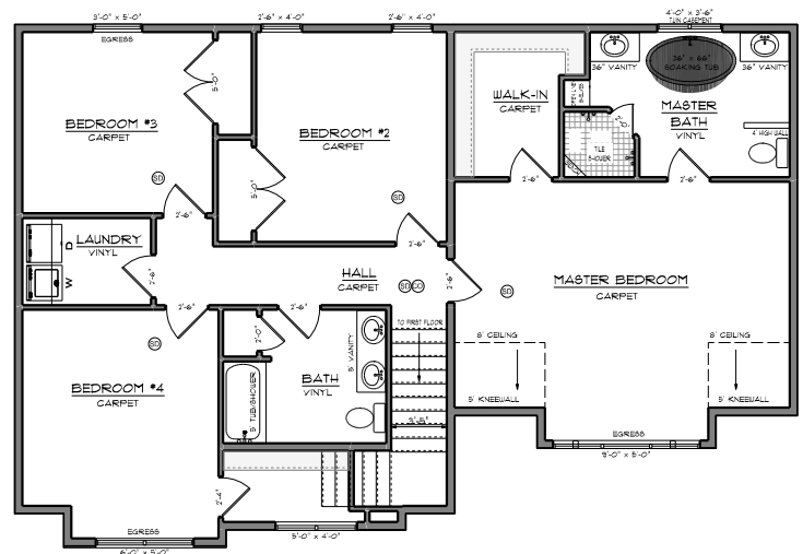
MODEL D SECOND FLOOR PLAN 1,365 SQ. FT.
