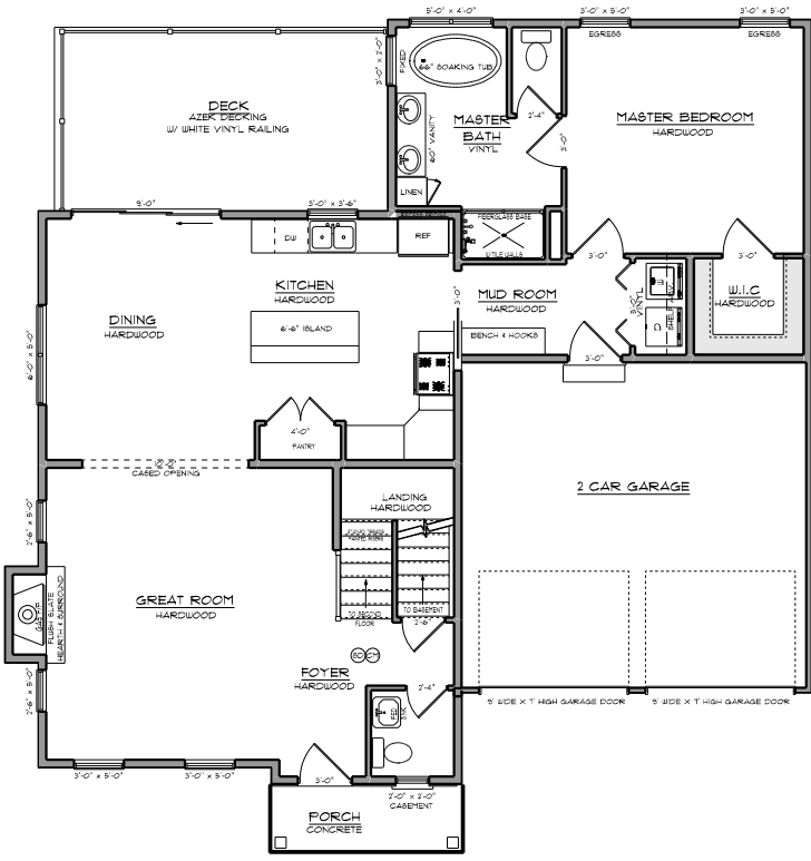
MODEL E FIRST FLOOR PLAN 1,350 SQUARE FEET
