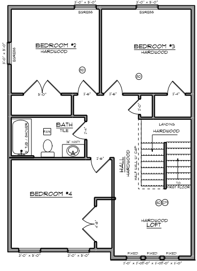
MODEL E SECOND FLOOR PLAN 870 SQUARE FEET
